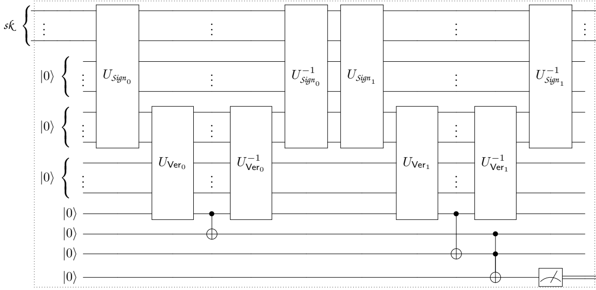
Figure 1: Quantum lightning from one-shot signatures. The verification algorithm. Here U_A corresponds to the unitary operator implementing the algorithm A without any final measurement. Moreover, Sign_b and Ver_b correspond to signing the bit b and verifying the signature of the bit b , respectively.
